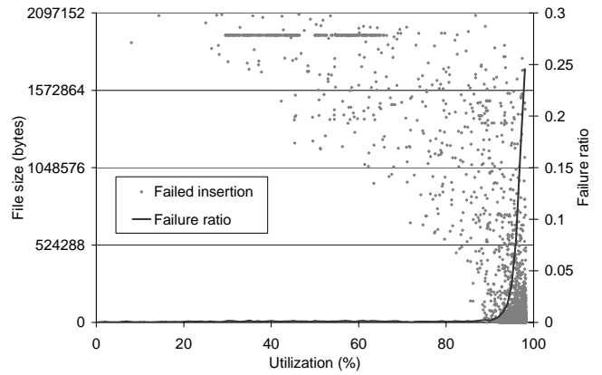
Figure 6: File insertion failures versus storage utilization for the NLANR trace, when t_{pri} = 0.1 , t_{div} = 0.05 .
